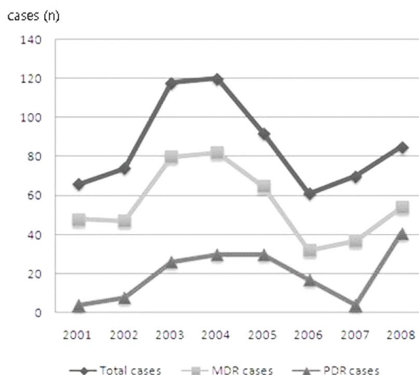
Fig. 1. This figure shows the incidence of total, MDR (multi-drug resistant), and PDR (pan-drug resistant) Acinetobacter baumannii infection. Note the sudden drop of curves after 2005, when our hospital changed the old intensive care unit to a new one due to the opening of a new hospital. However, incidences have increased since that time.
