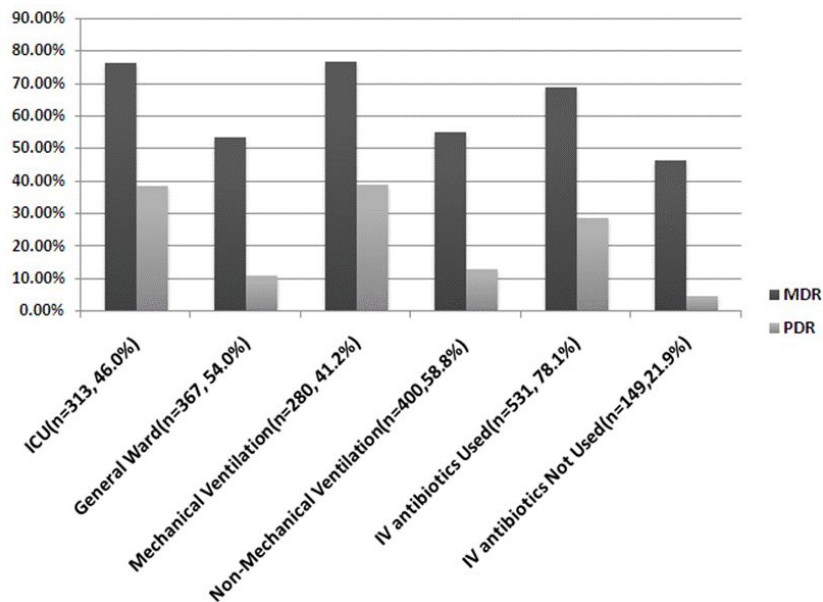
Fig. 2. This figure shows the relationship between the admitted location, mechanical ventilation, intravenous antibiotic use, and incidence of MDR or PDR.
