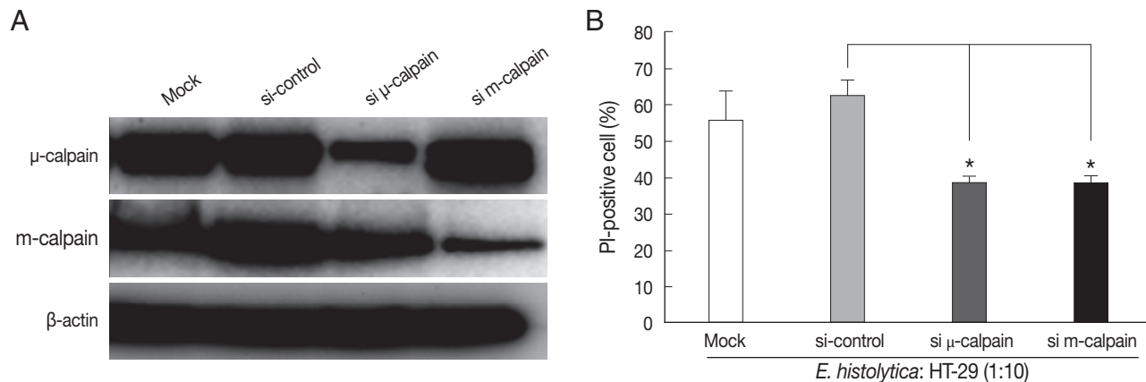
Fig. 2. siRNA-mediated knockdown of m-calpain or \mu -calpain inhibits E. histolytica -induced cell death in HT-29 colon epithelial cells. (A) Analysis of m- or \mu -calpain protein levels using immunoblotting following knockdown of calpain by siRNA in HT-29 cells. At 72 hr post-transfection, whole-cell lysates from HT-29 cells transfected with vehicle alone (Mock), control scrambled siRNA (80 nM), or m or \mu -calpain siRNA (80 nM) were subjected to immunoblotting with Ab to m- or \mu -calpain. \beta -actin was used as an equal loading control. (B) Effects of m- or \mu -calpain siRNA on E. histolytica -induced cell death in HT-29 cells. At 72 hr post-transfection, HT-29 cells ( 4 \times 10^6 ) transfected with vehicle alone (Mock), control scrambled siRNA or m- or \mu -calpain siRNA were incubated with E. histolytica ( 4 \times 10^5 ) for 1 hr. Host cell death was measured using PI staining for flow cytometry analysis. Data are expressed as the mean \pm SEM of 3 experiments.
