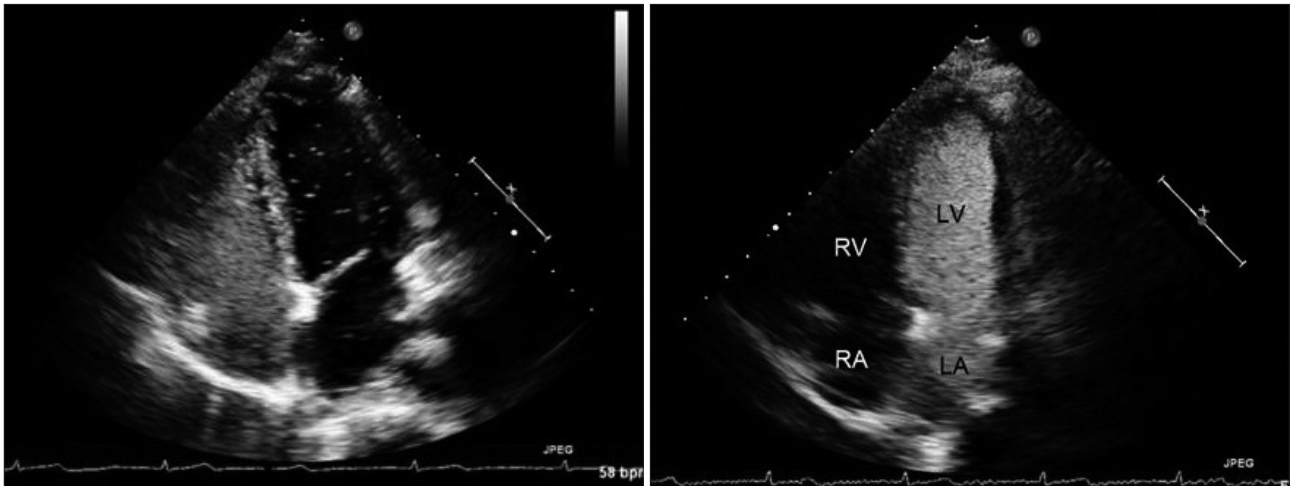
Fig. 1. Agitation saline injection test. On contrast echo conducted on Rt. arm, the enhancement was seen at not only Rt. side of heart, but also Lt. side. Sequential filling of the bubble in the left atrium followed by left ventricle and then through the patent foramen ovale to the right atrium. On Lt. arm contrast echocardiography, massive amount of microbubbles draining straight to LA was detected. LA: left atrium, LV: left ventricle, RA: right atrium, RV: right ventricle.
