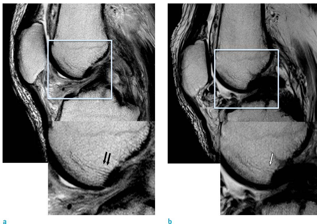
Fig. 2. (A) The thick, prominent, anisotropic trabecular bone pattern at the posterior cruciate ligament (PCL) femoral attachment site is apparent in the acute injury group (black arrows). (B) In contrast, the trabecular pattern is less prominent and smoothed in the chronic injury group (white arrow).
