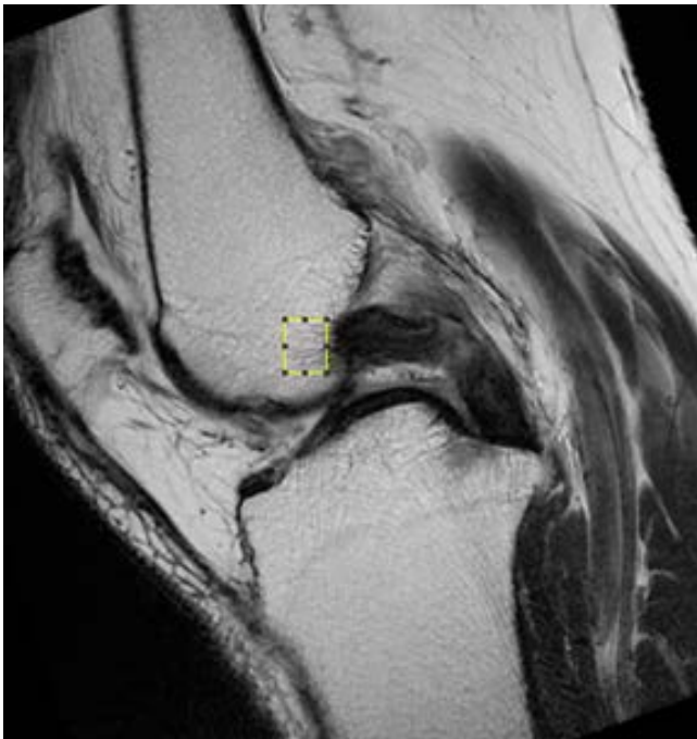
Fig. 1. Magnetic resonance (MR) image indicating a rectangular-shaped region-of-interest (ROI) measuring approximately 50 mm 2 at the bone, just near the posterior cruciate ligament (PCL) femoral attachment site.
