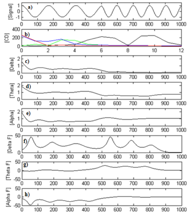
Fig. 5 Complex demodulation of synthetic data of 6 Hz and 10 Hz center frequencies. (a) ~ (e) are the same as Fig. 4
