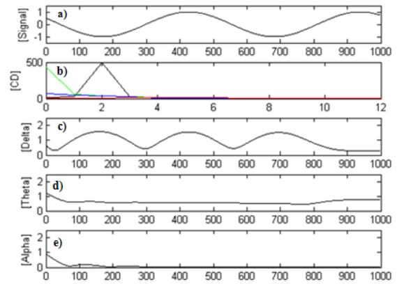
Fig. 1 Complex demodulation of synthetic data of 2 Hz center frequency. (a) synthetic signal, (b) power spectral density (black for original data, green for shifted delta, blue for shifted theta, and red for shifted alpha), (c) delta amplitude, (d) theta amplitude, and (e) alpha amplitude
