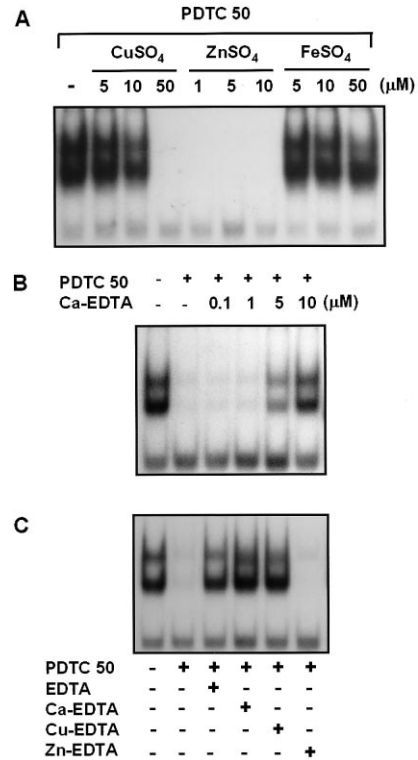
Fig. 2. Effects of selected metals on PDTC inhibition of NF-κB activity. A: BCECs were treated with various concentrations of CuSO 4 , FeSO 4 or ZnSO 4 , plus PDTC (50 μM) for 4 h after serum withdrawal. B: PDTC was co-administered with the indicated concentrations of Ca-EDTA to BCECs grown in the DMEM containing 10% FBS. C: Free base, Ca-, Cu- or Zn-EDTA (each 10 μM) and PDTC (50 μM) were added together to BCECs grown in DMEM containing 10% FBS.
