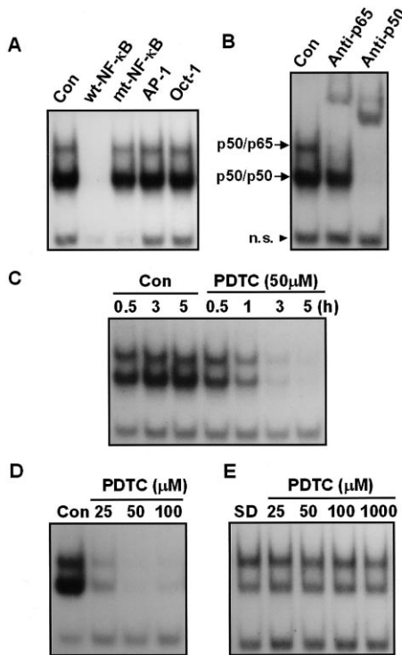
Fig. 1. Effect of PDTC on NF-κB activation in BCECs. Nuclear extracts were obtained 4 h after PDTC or vehicle treatment followed by EMSA. Basal NF-κB activity was present in BCECs grown in DMEM containing 10% FBS (Con). A: Competition for NF-κB binding with cold nucleotides (wild-type (wt-) or mutant (mt-) NF-κB, AP-1 or Oct-1) which were in excess of 100-fold. B: Supershift with anti-p65 or anti-p50 IgG. Arrowhead denotes the non-specific band (n.s.). C: A time course of NF-κB inhibition by PDTC (50 μM). D: Dose-dependent inhibition of NF-κB by PDTC in DMEM containing 10% FBS. E: Lack of PDTC effect on NF-κB activity in serum-deprived BCECs.
