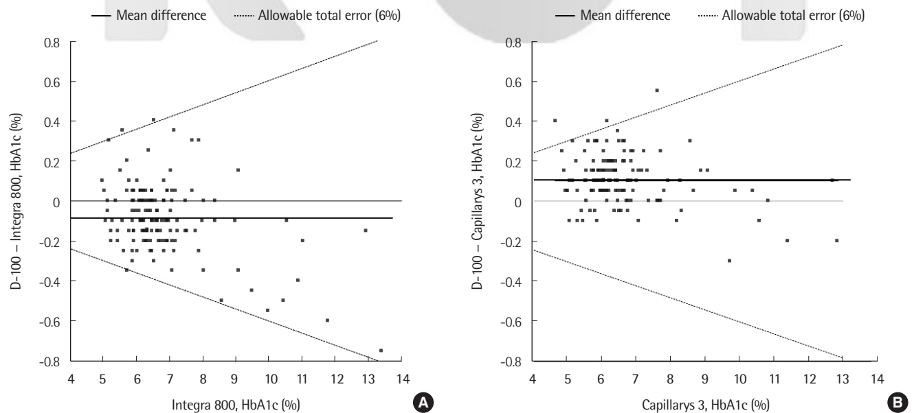
Fig. 3. A Bland-Altman difference plot for D-100 and Integra 800 (A) and for D-100 and Capillary 3 (B).
