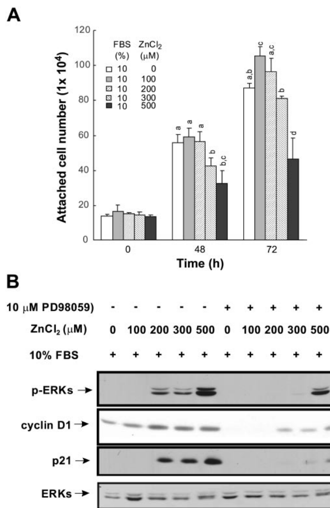
Fig. 6. Positive and negative regulations of cell growth and the differential activation of ERK and induction of p21 Cip/WAF1 in 10% FBS medium by ZnCl 2 at concentrations > 100 \mu M ZnCl 2 . A: experiments are as in Fig. 1B except that higher ZnCl 2 concentrations (0, 100, 200, 300, and 500 \mu M) were used. Values are means \pm SD of 3 independent experiments. Means with different lowercase letters are significantly different at P < 0.05 . B: experiments are essentially the same as in Fig. 5, except that a broader range of ZnCl 2 concentrations (0, 100, 200, 300, or 500 \mu M) was used. When required, 10 \mu M PD-98059 was added 1 h before zinc treatment. Cells were harvested at 9 h after treatment with zinc for Western blot analysis.
