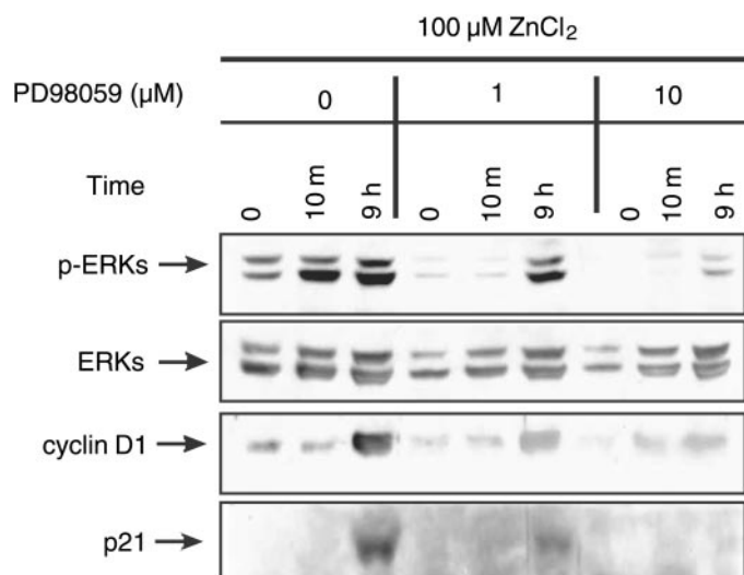
Fig. 4. Effects of PD-98059 on cyclin D1 and p21 Cip/WAF1 induction. Serum-starved HT-29 cells grown in MSSM were treated with 100 \mu M ZnCl 2 . Cells were incubated with 1 or 10 \mu M PD-98059 for 1 h before zinc treatment. Cells were then harvested, and Western blot analysis was performed as described in Fig. 3A.
