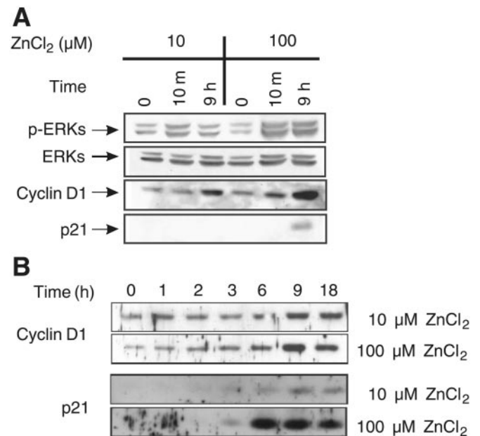
Fig. 3. ERK activations and inductions of cyclin D1 and p21 Cip/WAF1 by 10 and 100 \mu M ZnCl 2 . A: serum-starved HT-29 cells grown in MSSM were treated with 10 or 100 \mu M ZnCl 2 . The cells were then harvested at different time points (0 min, 10 min, and 9 h), and Western blot analysis was performed using phospho-ERK (p-ERK), ERK, cyclin D1, or p21 Cip/WAF1 (p21) antibodies. B: same experiment as in A except that samples were harvested over a greater period of time to detect cyclin D1 or p21 Cip/WAF1 .
