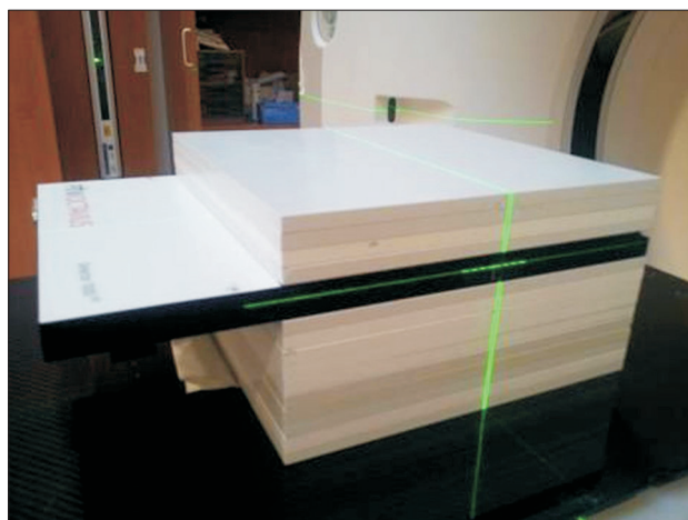
Fig. 2. Patient-specific QA phantom including fiducial-inserted solid water phantom and Octavius 1000SRS detector.
