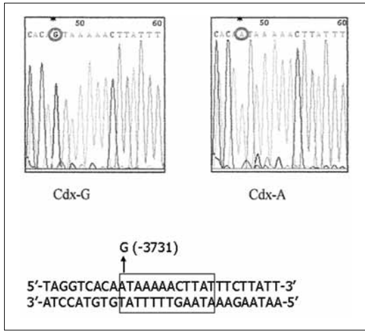
Fig. 1. Sequence determination on the polymorphism site in the promoter of the hVDR gene. Sequence data showed that Cdx-A allele is 5'-ATAAAA-CTTAT-3' in the Cdx-2 binding site, while the Cdx-G allele is 5'-GTAAAACCTTAT-3' in the Cdx-2 binding site.
