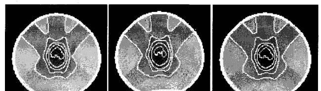
Fig. 5. Repeated gel dosimetry: Coronal view. Each gel showed different gel response but the resultant dose distribution were identical. The isodose lines are 20%, 40%, 60%, 80%, and 100% and outer line indicates 20% isodose.
