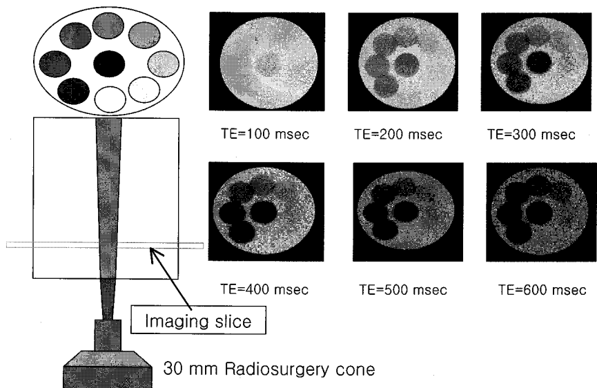
Fig. 2. Gel phantom irradiation scheme and MR images of different echo times. The imaging plane was set to SAD=100 cm position and irradiated using 6 MV X-ray.
