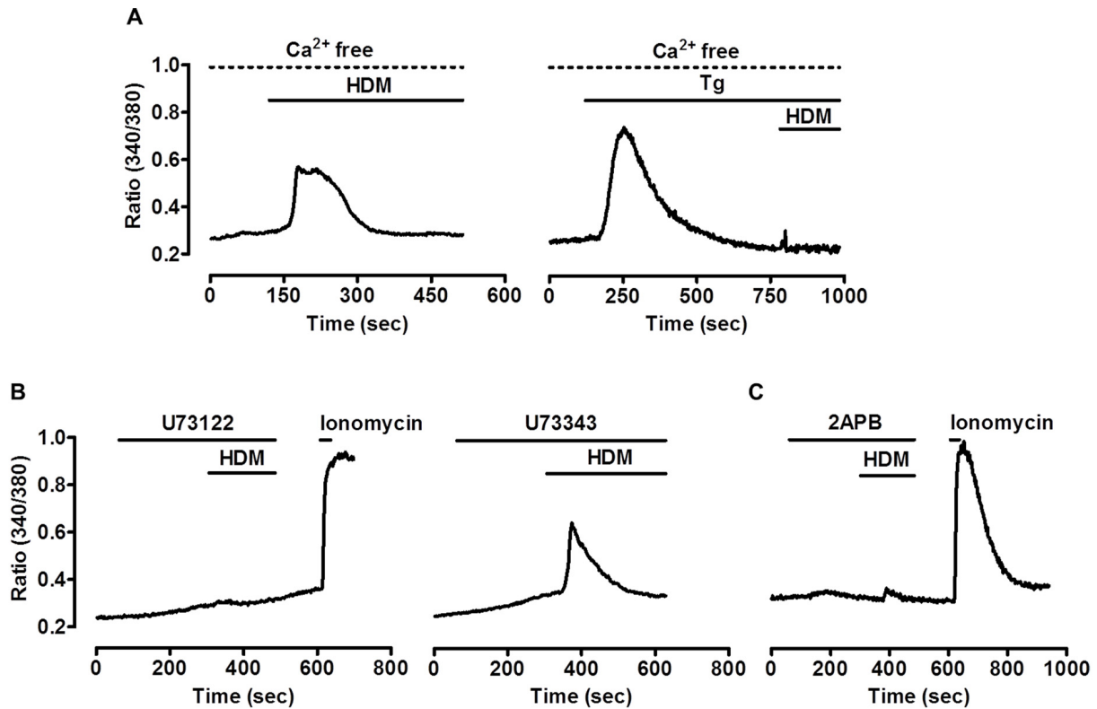
Fig. 2. HDM extract triggers PLC/IP 3 dependent Ca 2+ signaling in human gingival epithelial cells. (A) Effects of extracellular Ca 2+ depletion or thapsigargin (Tg) treatment on HDM extract-induced increase in [Ca 2+ ] i . The change in [Ca 2+ ] i in response to HDM extract was measured after the pre-treatment of a Ca 2+ -free PPS or Tg (1 μM) in a Ca 2+ -free PPS. (B) Effects of U73122 or U73343 treatment on HDM extract-induced increase in [Ca 2+ ] i . The change in [Ca 2+ ] i in response to HDM extract was measured after the pre-treatment of U73122 (10 μM) or U73343 (10 μM) in PPS. Ionomycin was used as a positive control. (C) Effect of 2-aminoethoxydiphenyl borate (2-APB) treatment on HDM extract-induced increase in [Ca 2+ ] i . The change in [Ca 2+ ] i in response to HDM extract was measured after the pre-treatment of 2-APB (75 μM) in PPS.
