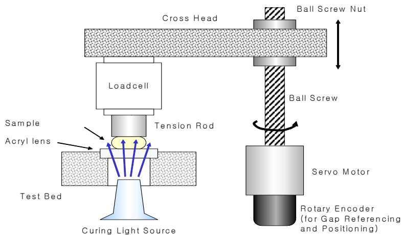
Fig. 1. Schematic drawing of the custom made polymerization shrinkage stress measuring machine with a sample in place.
