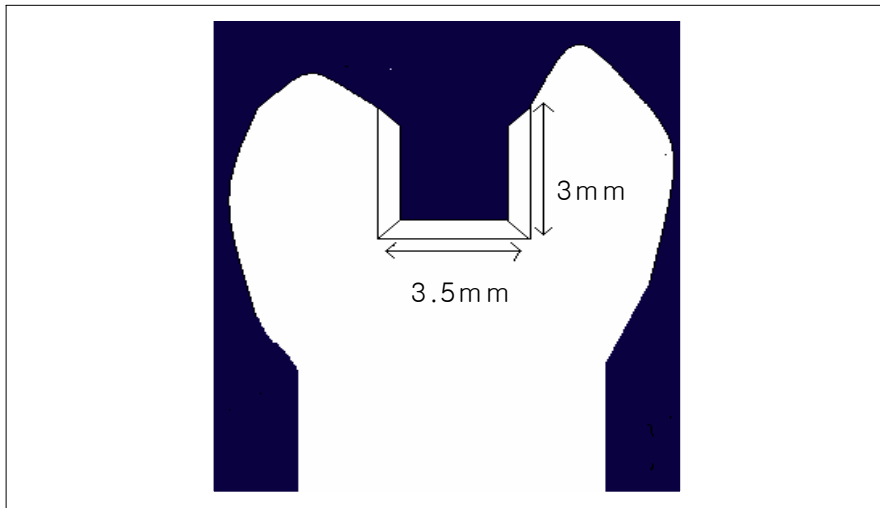
Fig. 2. Schematic drawing of cavity preparation.
