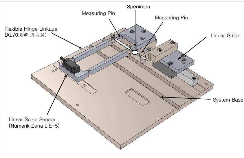
Fig. 3. cuspal deflection measuring machine.
