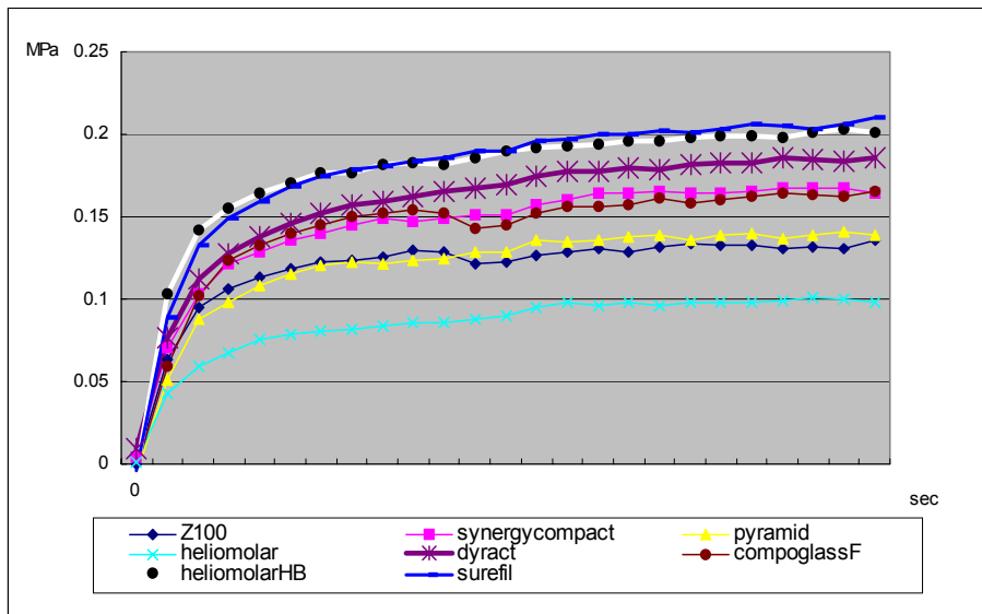
Fig. 5. Change in the polymerization stress versus time.
