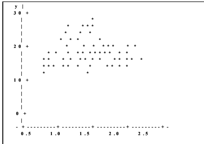
Fig. 7. Regression analysis
