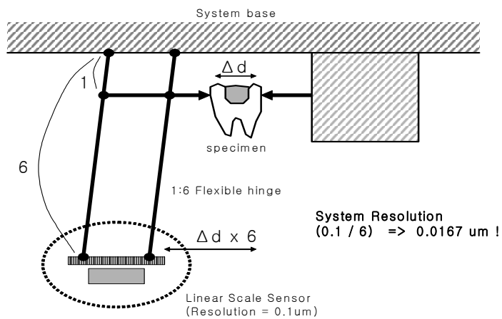
Fig. 4. Schematic drawing of the cuspal deflection measuring machine.
