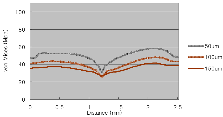
Fig. 5 von Mises stress at Tetric Flow when lingual loading applied
