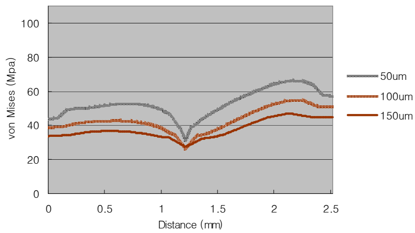
Fig. 3 von Mises stress at Tetric Flow when buccal loading applied
