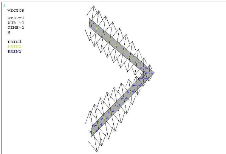
Fig. 6 Principal stress vectors on adhesive when buccal loading applied
