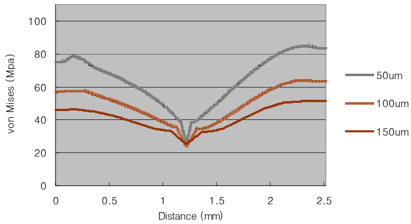
Fig. 4 von Mises stress at Z100 when lingual loading applied
