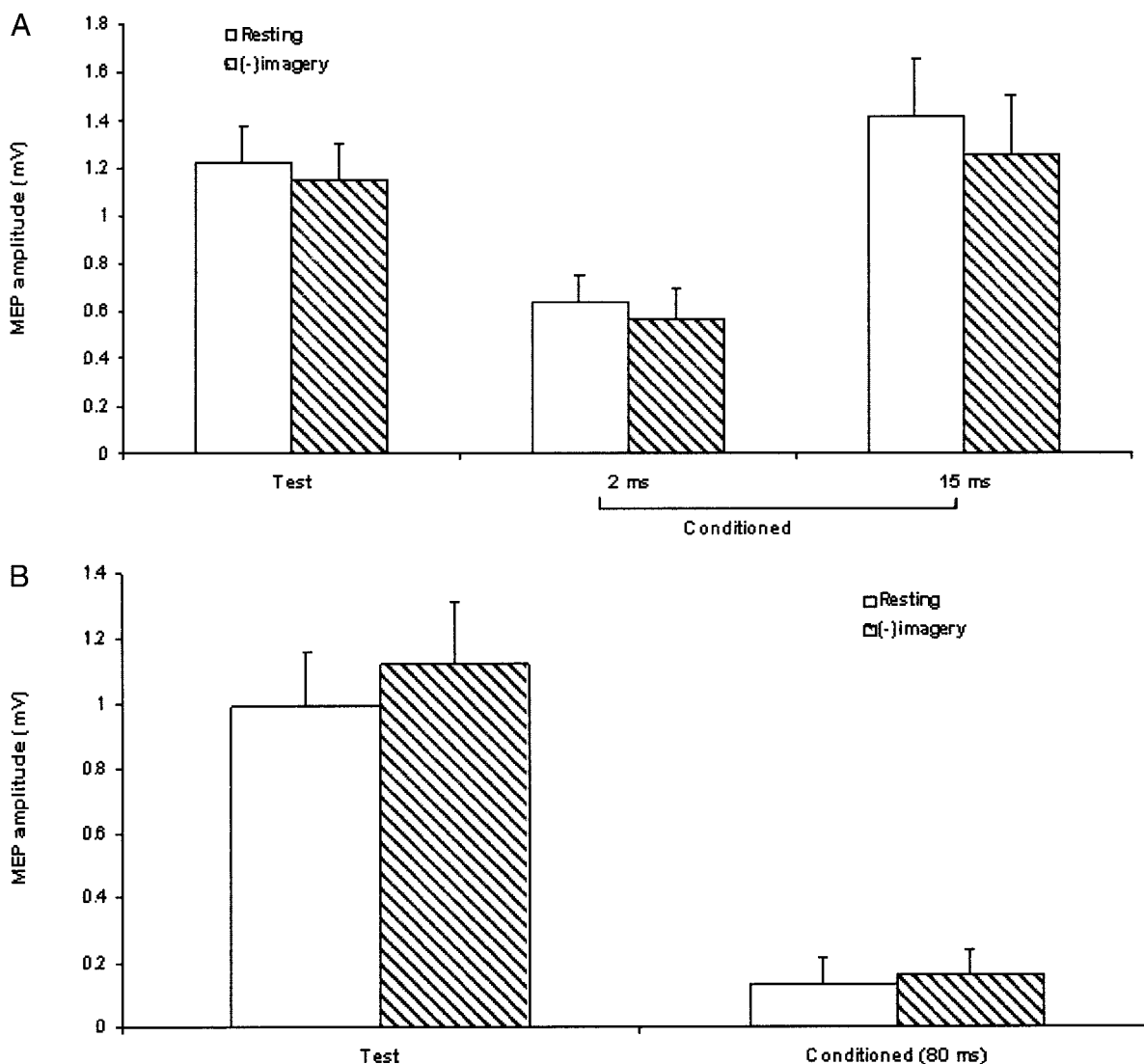
FIG. 3. Average MEP amplitudes (mV) of the FDI produced by conditioning and test stimuli in negative motor imagery and control conditions. A : short intracortical inhibition and intracortical facilitation used subthreshold conditioning stimulus (70% resting motor threshold) and suprathreshold test stimulation ( MT_{1mV} ) at 2- and 15-ms interstimulus intervals. Test and conditioned MEP amplitudes at both interstimulus intervals were comparable between the two conditions. B : long intracortical inhibition employed suprathreshold conditioning and test stimulation ( MT_{1mV} ) at interstimulus interval of 80 ms. Both test and conditioned MEP amplitudes were comparable for negative motor imagery and control conditions.
