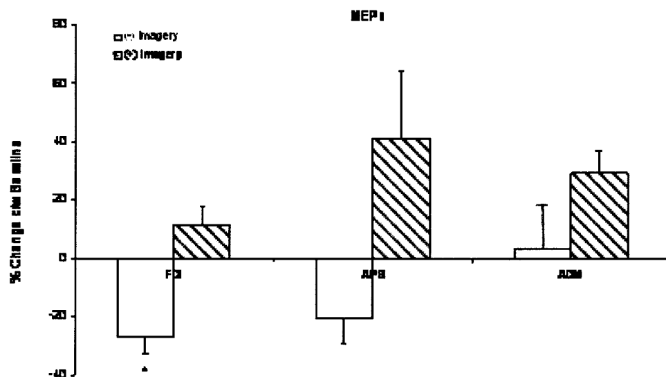
FIG. 1. Motor-evoked potential (MEP) amplitude change (%) in negative and positive motor imagery compared with control condition. Stimulation intensity was 140% resting motor threshold. Asterisks represent significant difference from control. During negative motor imagery, MEP amplitudes were significantly reduced in the 1st dorsal interosseus (FDI) and tended to be suppressed in abductor pollicis brevis (APB) muscles, while those were enhanced, although statistically insignificant, in all tested muscles during positive motor imagery.
