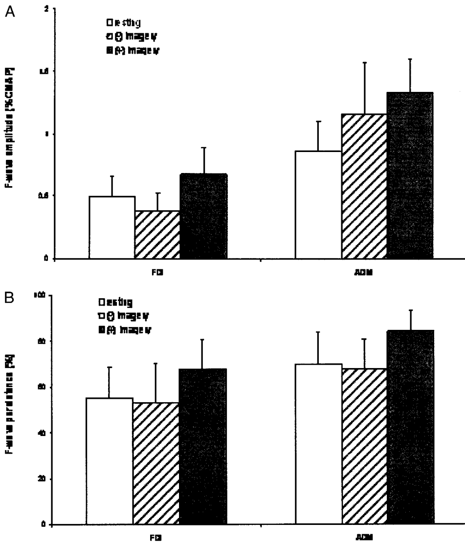
FIG. 2. F-wave amplitude (A) and persistence (B) during negative and positive motor imagery compared with resting state. Supramaximal electrical stimulation was applied to the ulnar nerve at the wrist ( n = 18 in each subject). In both the FDI and abductor digiti minimi (ADM), there is no significant change in F-wave amplitude and persistence during negative and positive motor imagery compared with resting state.
