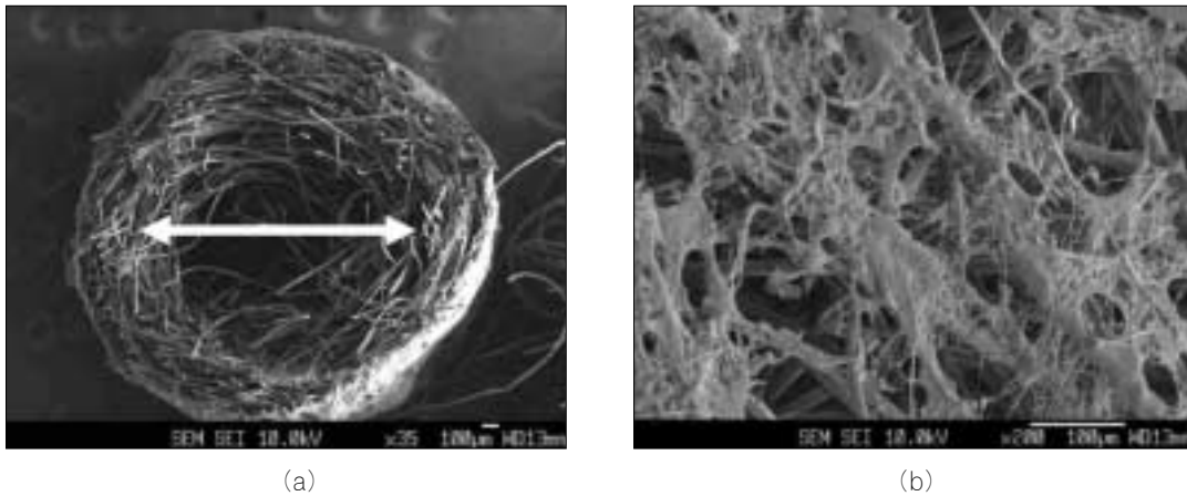
Fig. 3. (a) SEM photograph of PGA tube. Woven 12\mu\text{m} fiber is visible. Internal diameter was 1.5 to 1.8 mm (Internal Diameter : \leftrightarrow ). Inner fiber was soft enough to hold rat sciatic nerve end which diameter was between 1.0 and 1.5 mm. (b) 75:25 poly(lactic-co-glycolic acid) solution coated PGA mesh
