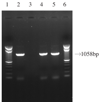
Fig. 1. Detection of amplified products of bla OXA-23 genes after 2% agarose gel electrophoresis. Lanes: 1 and 6, DNA molecular weight markers (X174 DNA/ Hae III Markers, Promega); 2, Positive control, OXA-23-producing A. baumannii ; 3, Negative control, imipenem-susceptible A. baumannii ; 4 and 5, Clinical isolates of A. baumannii resistant to imipenem and showed positive results in modified Hodge test.
