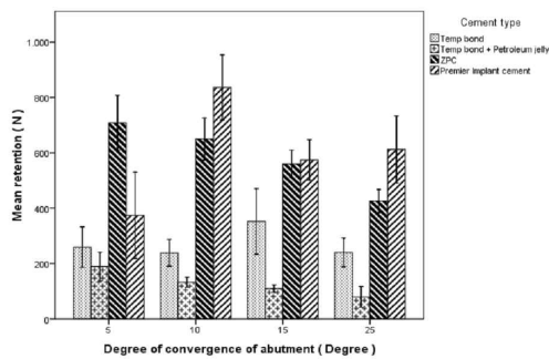
Fig. 4. Means and standard deviation of retention(N) for 5mm abutment length according to cement type (n=10)
