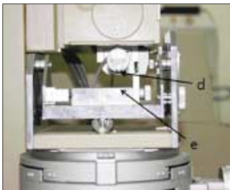
Fig. 1. Profilometer (a. vertical movement handle, b. set meter, c. rolling leg, d. stylus, e. fixation jig)
