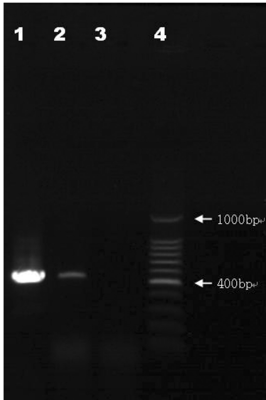
Fig. 2. Analysis of ITS PCR. Lane 1, dematiaceous fungi; lane 2, C. albicans ATCC 18804; lane 3, S. aureus ATCC 25923; lane 4, size marker.
