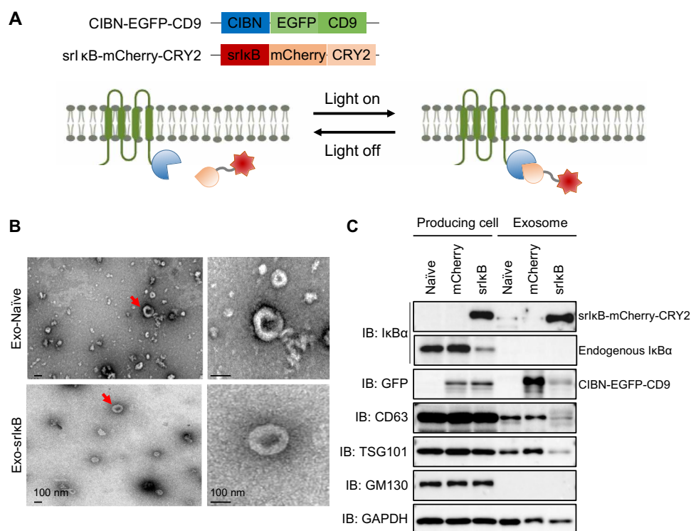
Fig. 1. Generation and characterization of engineered exosomes. (A) Schematic of DNA constructs used for the production of Exo-srIkB (top). Schematic showing fusion proteins and their proposed activities (bottom). (B) Morphological characterization of Exo-Naïve and Exo-srIkB through transmission electron microscopy. (C) HEK293T cells that stably express mCherry or srIkB, and exosomes from these HEK293T cells, were lysed and immunoblotted against the indicated proteins. IB, immunoblot.
