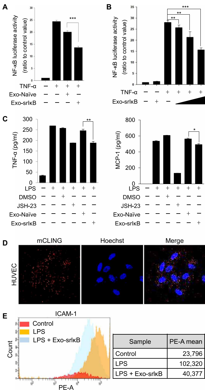
Fig. 4. Inhibitory effect of Exo-srIκB on NF-κB signaling in vitro. (A) HEK293–NF-κB–luciferase cells ( 2 \times 10^4 cells) were cultured either with Exo-Naive or with Exo-srIκB ( 2 \times 10^5 particles). After 24 hours, the cells were treated with TNF-α (0.5 ng/ml) for an additional 18 hours. Luciferase activities were measured and normalized. (B) Exo-srIκB dose-dependently repressed NF-κB activation in NF-κB–luciferase cells. (C) THP-1 cells ( 5 \times 10^5 cells) were stimulated with LPS (1 μg/ml) and then treated with Exo-srIκBs ( 5 \times 10^6 particles). The supernatants were collected and assayed for the production of TNF-α and MCP-1. JSH-23 (50 μM) was used as the positive control. ^{**}P < 0.01 . (D) Immunofluorescence of HUVECs incubated with mCLING-labeled Exo-srIκB. Representative images are shown. Nuclei were labeled with Hoechst. (E) HUVECs were stimulated with LPS (300 ng/ml) for 24 hours. Cells were harvested into a single-cell suspension and assessed through flow cytometry using specific phycoerythrin (PE)–conjugated antibodies against human ICAM-1. DMSO, dimethyl sulfoxide. ^{*}P < 0.05 ; ^{**}P < 0.01 ; ^{***}P < 0.001 .
