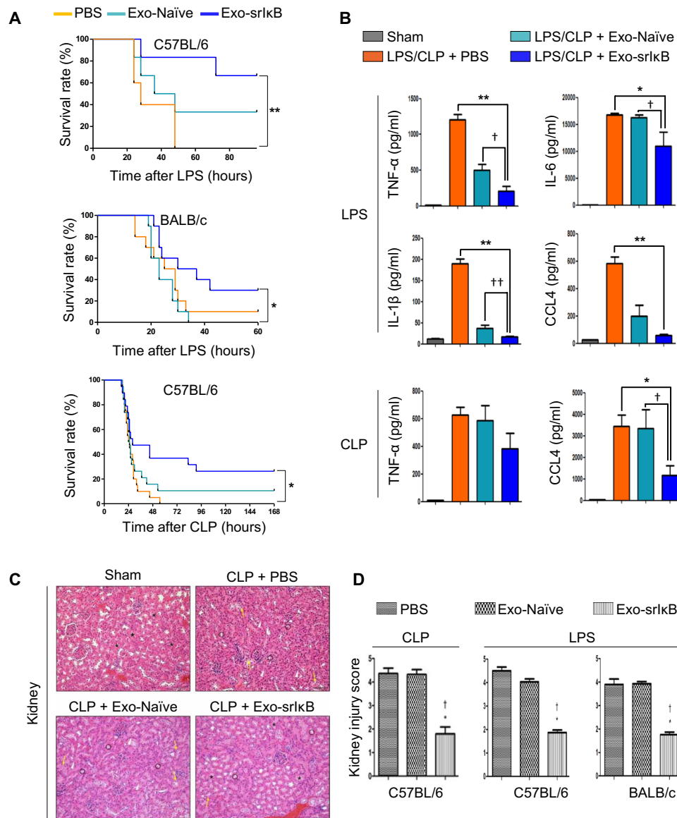
Fig. 2. The protective effects of Exo-srIkB in endotoxemia and CLP-induced sepsis. (A) Survival curves of phosphate-buffered saline (PBS)-, Exo-Naïve-, and Exo-srIkB-treated septic mice. LPS C57BL/6 mice ( n = 5 to 6 per group), LPS BALB/c mice ( n = 10 per group), and CLP C57BL/6 mice ( n = 14 to 15 per group). ** P < 0.01 and * P < 0.05 compared with the PBS-treated sepsis group. (B) Levels of TNF- \alpha , IL-6, IL-1 \beta , and CCL4/macrophage inflammatory protein-1 \beta in the plasma of exosome-treated mice were measured 24 hours after LPS injection or CLP. ** P < 0.01 and * P < 0.05 compared with the PBS-treated sepsis group. † P < 0.05 compared with the Exo-Naïve-treated sepsis group. (C) Representative images of cortical tubular cells in kidney sections from sham, CLP with PBS, CLP with Exo-Naïve, and CLP with Exo-srIkB mice. Normal brush border (*) of proximal tubules or loss of brush border (o), chromatin condensation (white arrows), denuded basement membrane (white arrow heads), and vacuolization (yellow arrows). Scale bars, 100 \mu M. (D) Pathological kidney injury scores of representative kidney samples of each group. * P < 0.05 compared with the PBS-treated sepsis group. † P < 0.05 compared with the Exo-Naïve-treated sepsis group. GFP, green fluorescent protein; GAPDH, glyceraldehyde-3-phosphate dehydrogenase.
