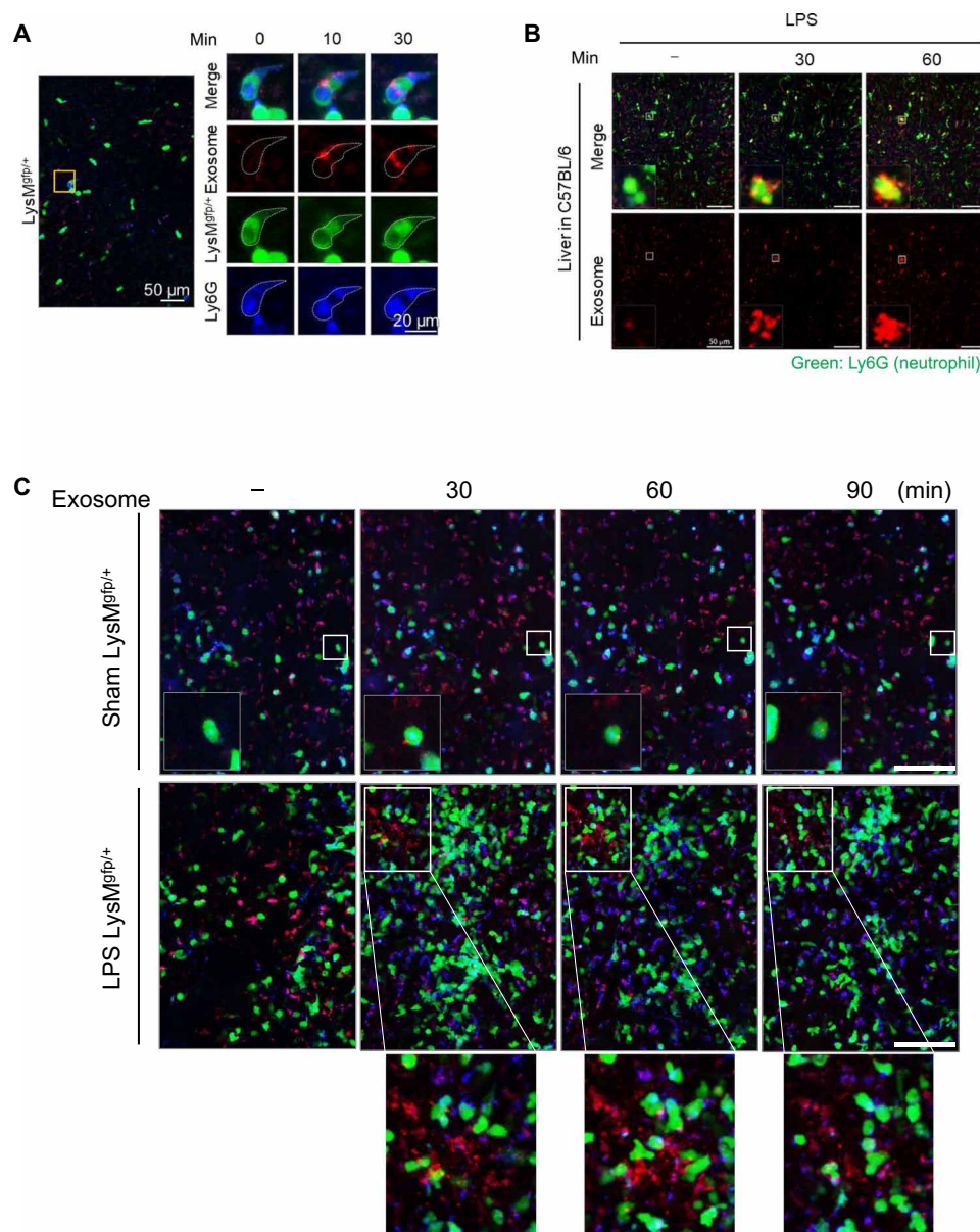
Fig. 3. The biodistribution of exosomes in LPS-injected mice. (A) Intravital imaging of mCLING-labeled exosome (red) uptake into neutrophils (LysM gfp/+ , green; Ly6G + , blue) in the liver of sham mice. (B) Representative time-lapse imaging of mCLING-labeled exosomes (red) inside the Ly6G + neutrophil cells (green) of the liver in LPS-treated C57BL/6 mice. (C) Sequential images of flowing mCLING-labeled exosomes (red) inside the spleen of sham- and LPS-treated LysM gfp/+ mice. Elapsed time is indicated. Magenta, autofluorescence. Scale bars, 50 \mu m.
