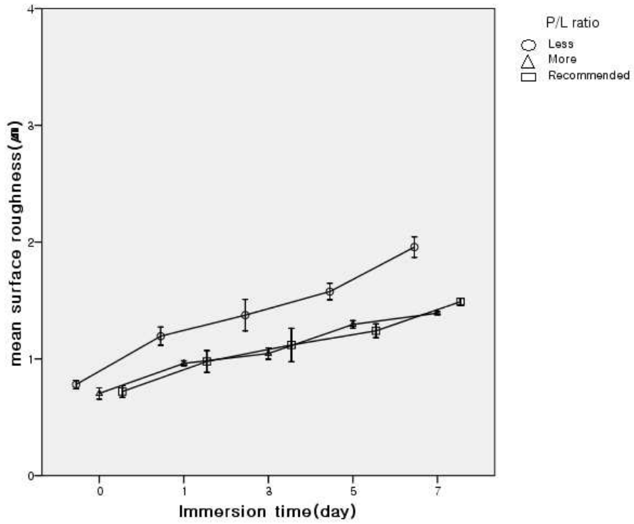
Fig 7. Comparison of mean surface roughness by P/L ratios at Visco-Gel.
