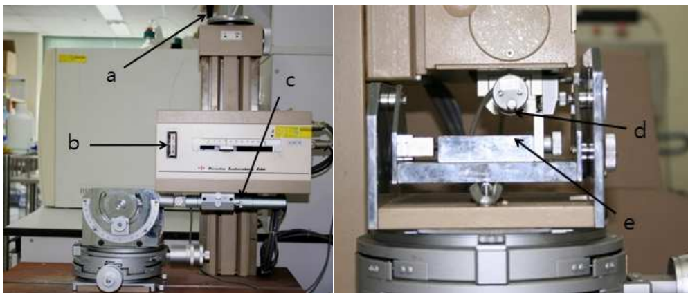
Fig 1. Profilometer (a. vertical movement handle, b. set meter, c. rolling leg, d. stylus, e. fixation jig)
