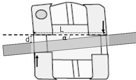
Fig. 4. Vertical force can be occurred at the end of bracket slot (2 vertical arrows) as wire is inclined into the slot.
